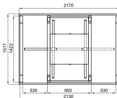
Dimensions (mm)
