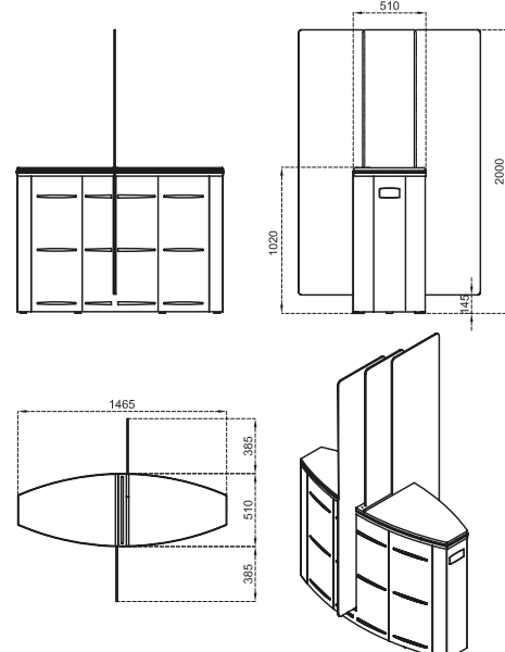
SG 90 T-C Glass Wing Height: 2000 mm
